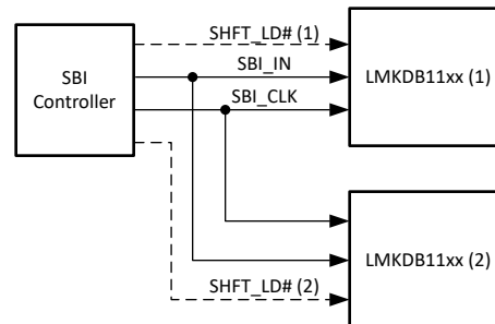
Figure 8-13. SBI Star Topology
