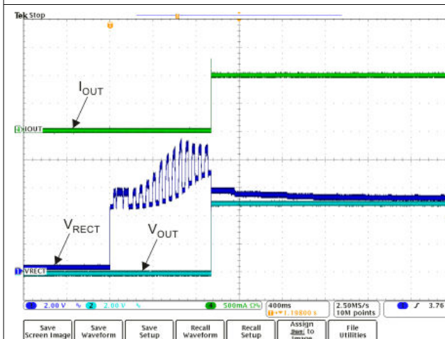
Figure 7-17. BQ51013C-Q1 Typical Start-Up With a 1-A System Load
