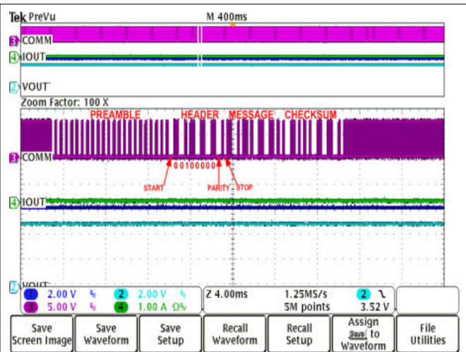
Figure 7-20. RX Communication Packet Structure
