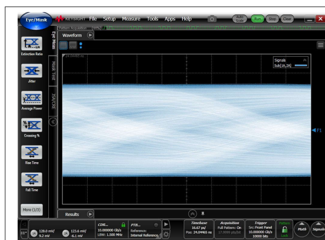
Figure 7-3. 10 Gbps Input Eye At SSTX After 12.5 dB at 5 GHz Pre-channel
