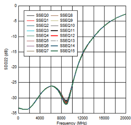
Figure 4-4. CTX1 Output Return Loss Performance at 85 \Omega (from simulation)
