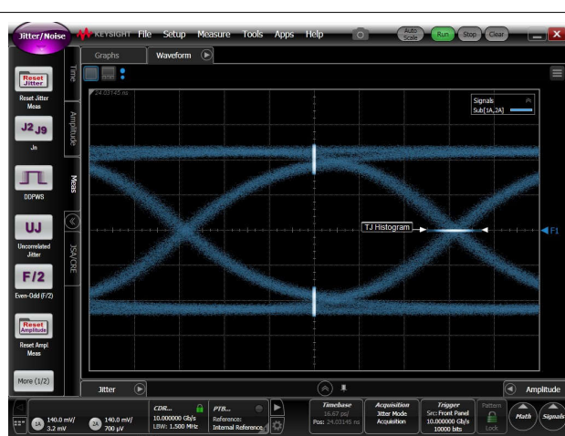
Figure 7-4. 10 Gbps Output Eye at CTX1 After 1.2 dB at 5 GHz Post-Channel
