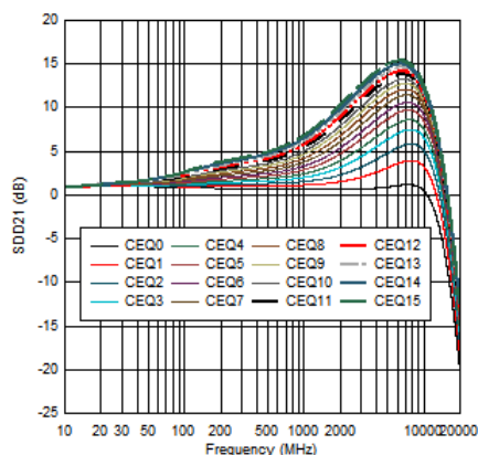
Figure 4-1. USB CRX1 EQ Settings Curves at 85 \Omega (from simulation)
