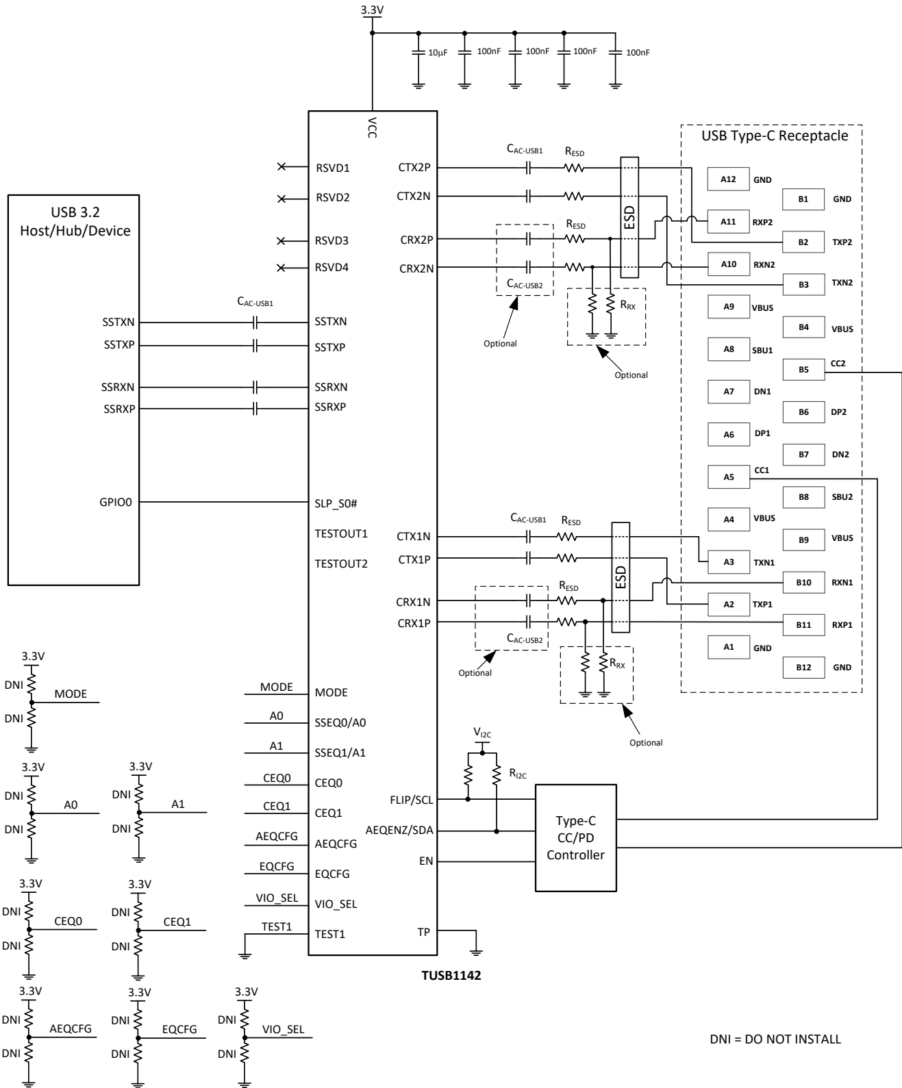
Figure 7-2. Application Circuit
