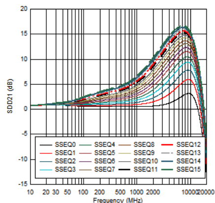
Figure 4-2. USB SSTX EQ Settings Curves at 85 \Omega (from simulation)
