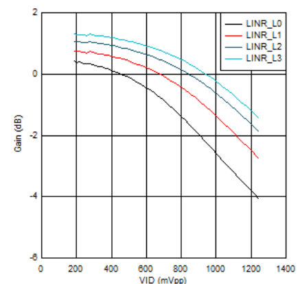
Figure 4-6. USB SSRX VOD Linearity Settings at 5 GHz and EQ = 0
