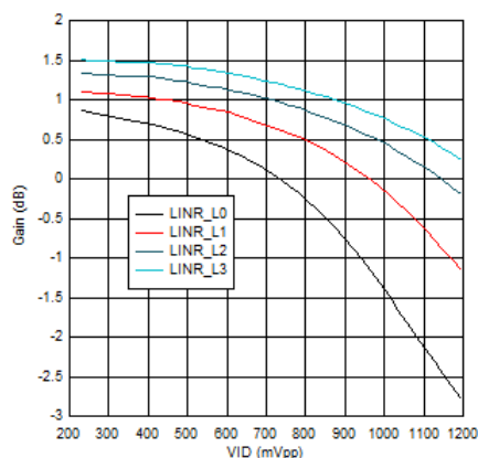
Figure 4-5. USB SSRX VOD Linearity Settings at 20 MHz and EQ = 0
