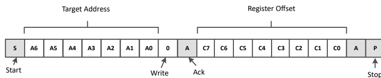
Figure 6-5. I2C Write Without Data
