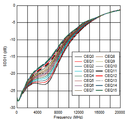
Figure 4-3. CRX1 Input Return Loss Performance at 85 \Omega (from simulation)
