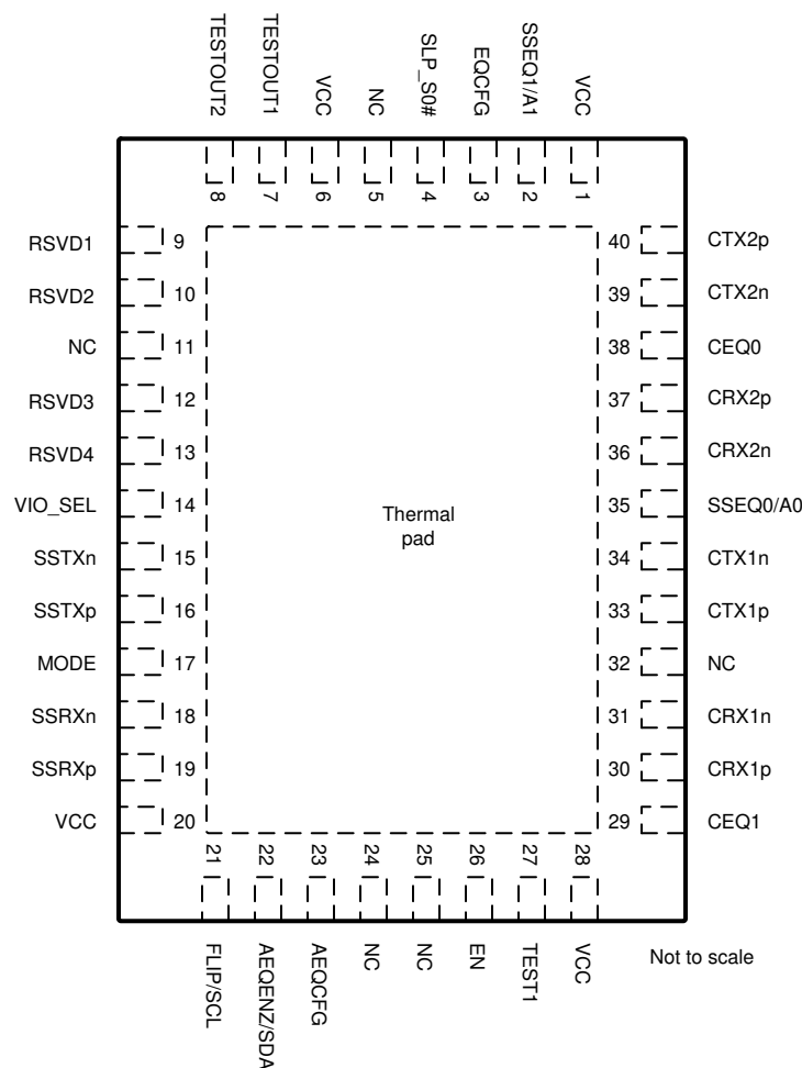
Figure 3-1. TUSB1142 RNQ Package, 40-Pin WQFN (Top View)
