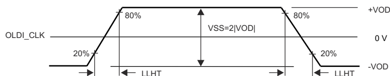
Figure 6-108. LVDS Output Transition Times
