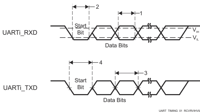
Figure 6-110. UART Timing
