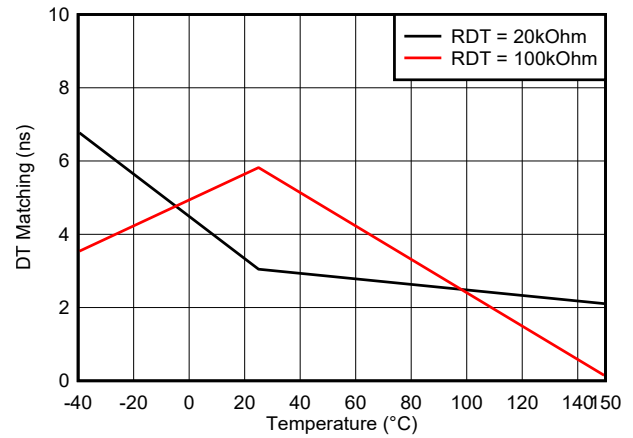
Figure 5-31. Dead Time Matching vs Temperature (with R_{DT} = 20\text{ k}\Omega and 100\text{ k}\Omega )
