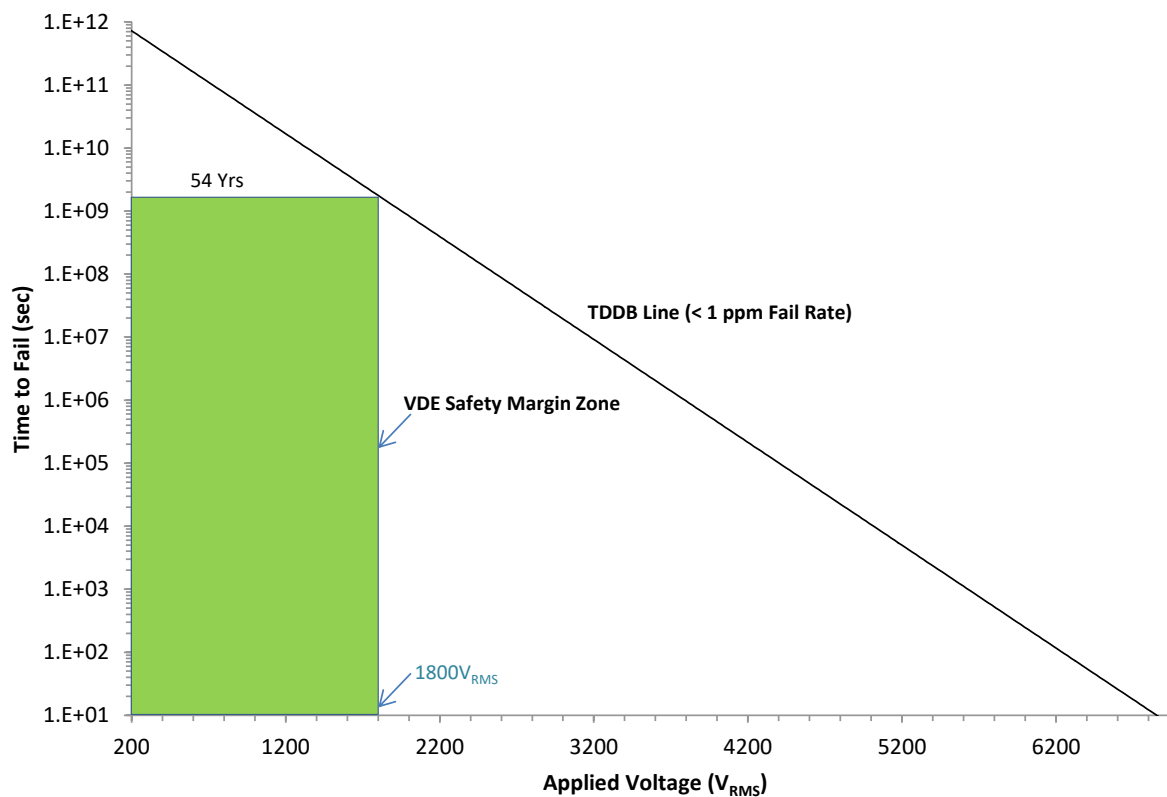
Figure 5-5. Reinforced Isolation Capacitor Life Time Projection
