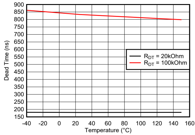
Figure 5-30. Dead Time vs Temperature (with R_{DT} = 20\text{ k}\Omega and 100\text{ k}\Omega )
