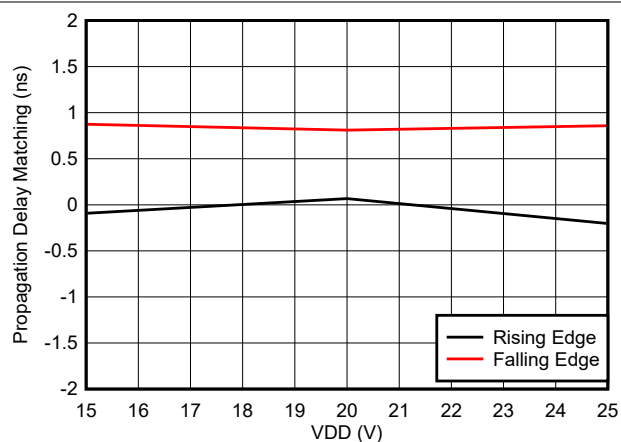
Figure 5-17. Propagation Delay Matching ( t_{\text{DM}} ) vs VDD
